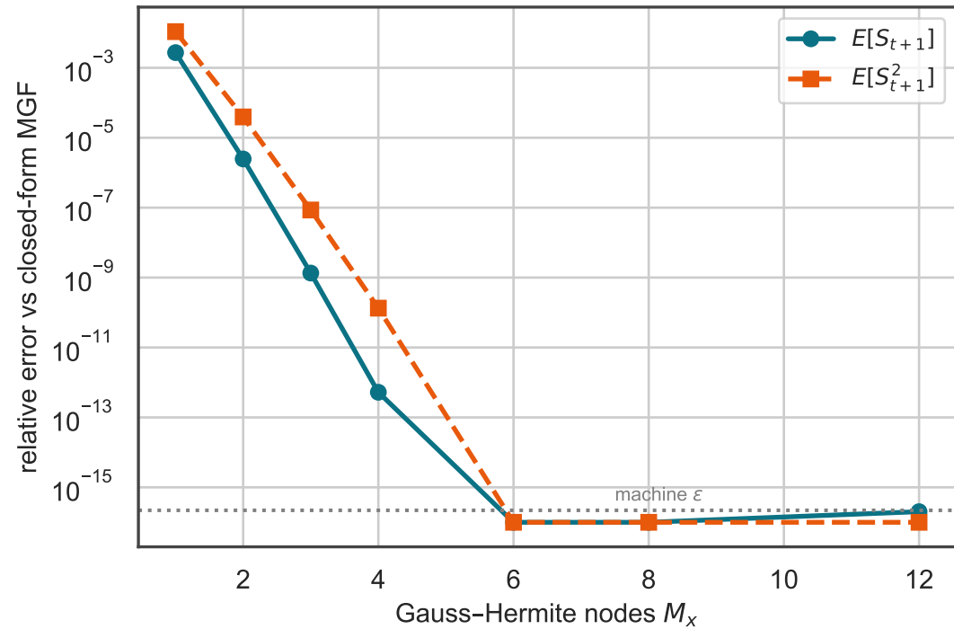
(a) OU/Gaussian leg — spectral convergence ( \lambda = 0 )
