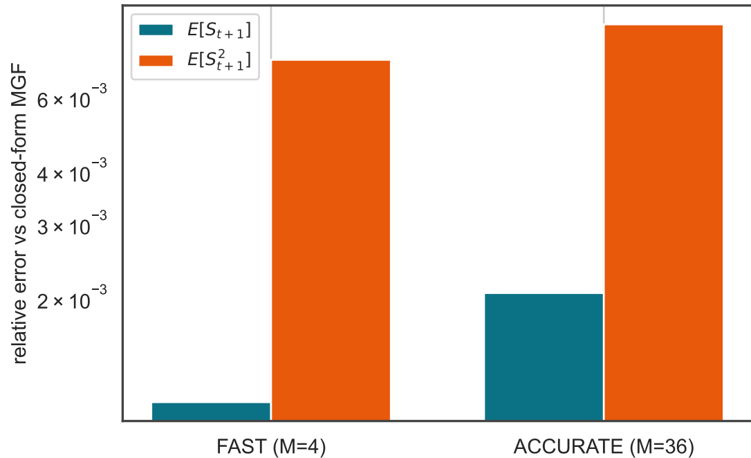
(b) Full kernel (with jumps) — moment error
